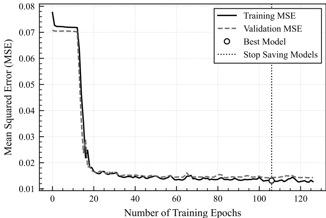
Learning Curve of TCSA-Transformer Model for SolarPlant-3 (Gyeongju)
